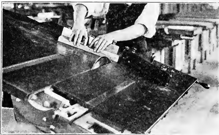
FIG. 164. SAWING COMPOUND MITERS.
